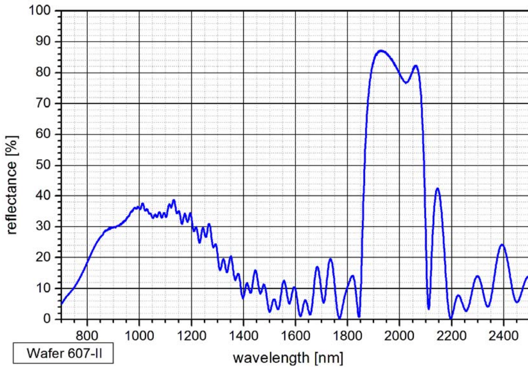
Wide range spectrum
