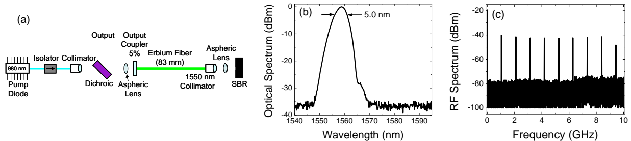
Fig.1.(a) Experimental set-up of Er fiber laser with a free space section; (b) Optical spectrum centered at 1559 nm with a 3-dB bandwidth of 5.0 nm; (c) RF spectrum with fundamental repetition rate of 1.047 GHz for a resolution bandwidth of 100 kHz.
