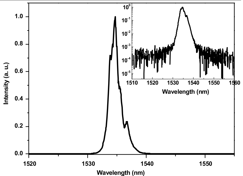
Fig. 3 Typical output spectrum of the output signal on a linear scale. Inset shows the optical spectrum on a logarithmic scale
