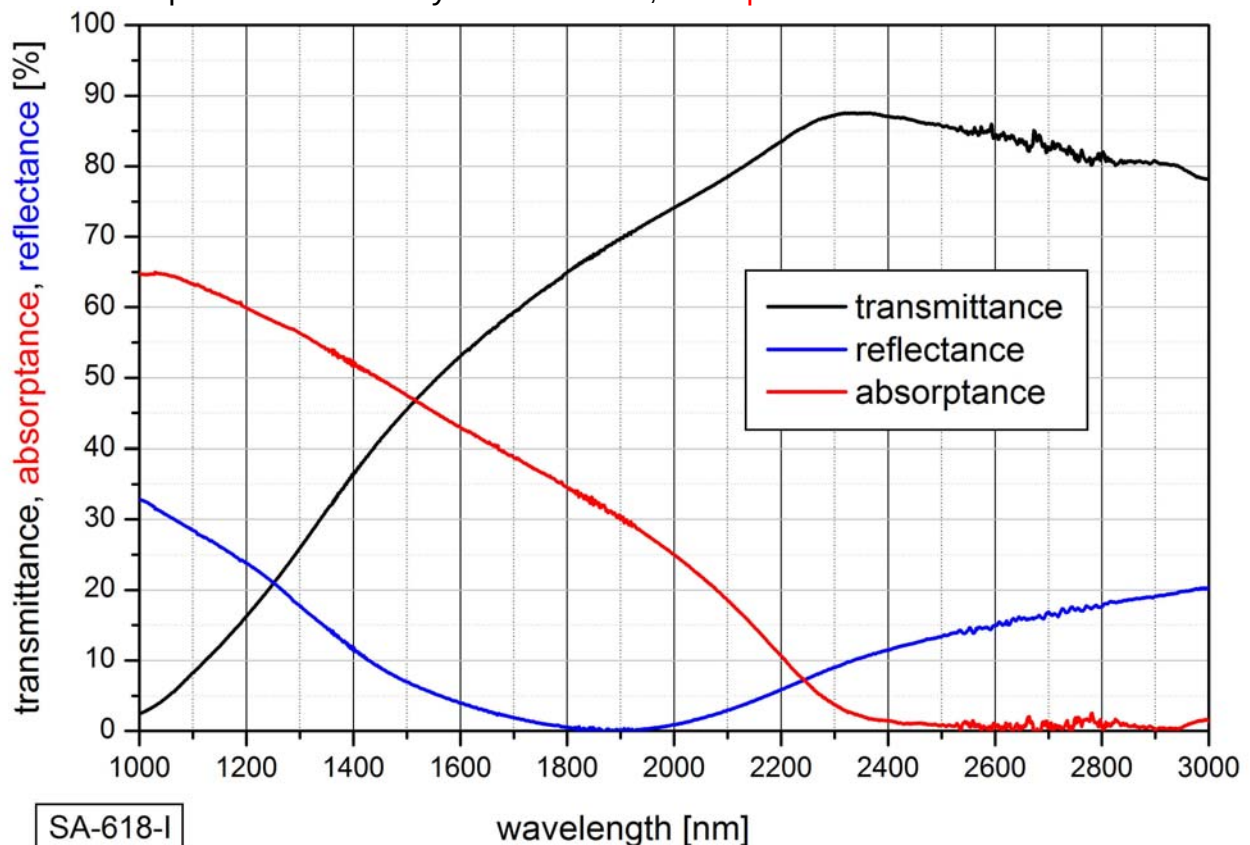
Spectral low intensity transmittance, absorptance and reflectance
